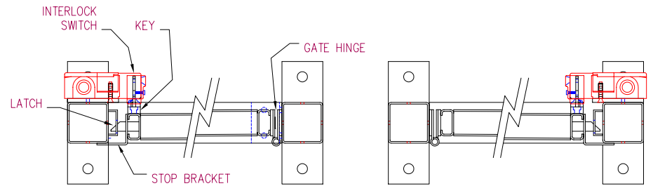
HINGE RIGHT; SWING OUT
