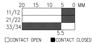
HINGE LEFT; SWING IN
