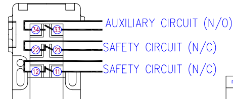
WIRING DIAGRAM
