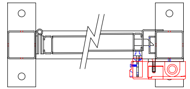
HINGE LEFT; SWING IN
